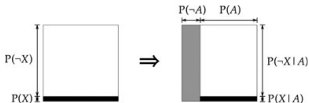
Figure 1. Meta-level uncertainty.
