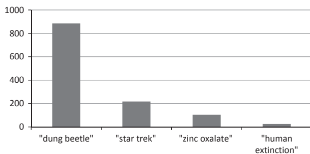
Figure 6. Academic prioritisation.
